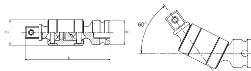
UNIVERSAL DOUBLE JOINT
